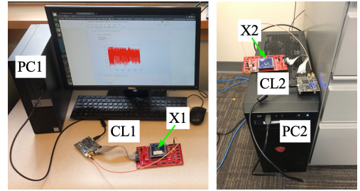
Figure 10: Our data collection setup (was also used in [39])
